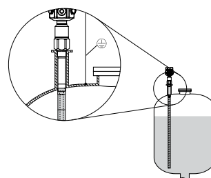
Figure 4: Installation in a nozzle
