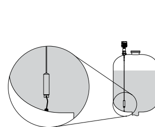
Figure 7: Tensioning weight
