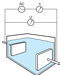
Figure 1: The principle of conductive measurement of conductivity AC Power supply I Current meter U Voltage meter
