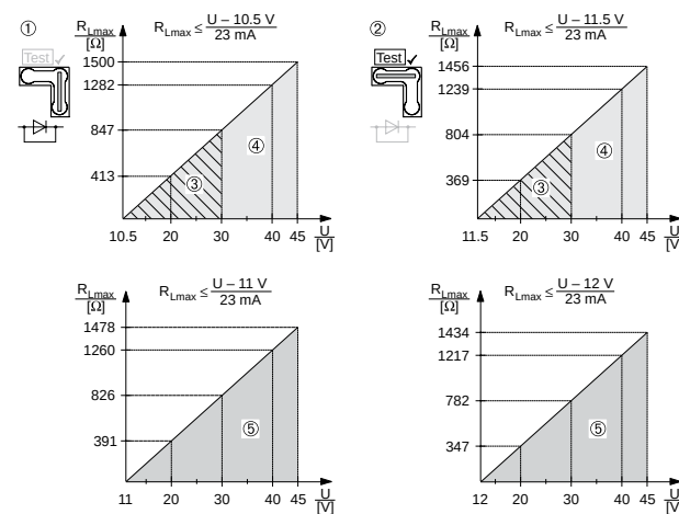
Figure 8: Load diagram
