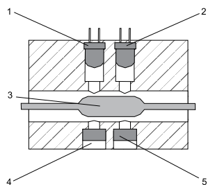
Figure 3: Stamolys analyzers design 1 Reference LED 2 Emitter LED 3 Sample 4 Reference detector 5 Measuring detector
