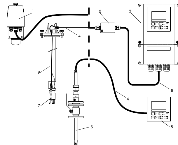
Figure 1: Example of a complete measuring system
