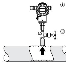
Figure 4: Measuring arrangement for pressure measurement in gases 1 Cerabar S 2 Shut-off device
