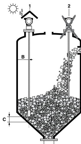
Figure 4: General installation conditions 1 = correct installation
