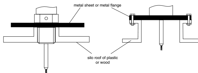
Figure 7: Installation in plastic containers
