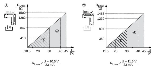
Figure 2: Load diagram
