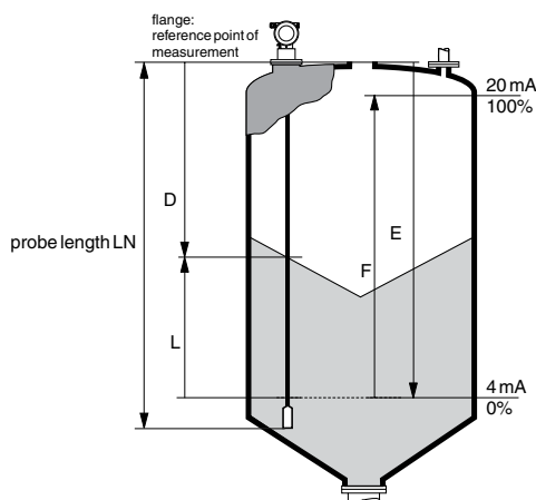
Figure 1: Measuring principle
