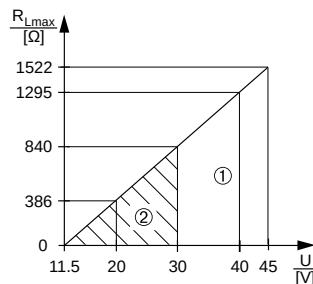
Figure 3: Load diagram
