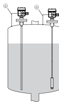
Figure 2: Installation on containers that conduct electricity
