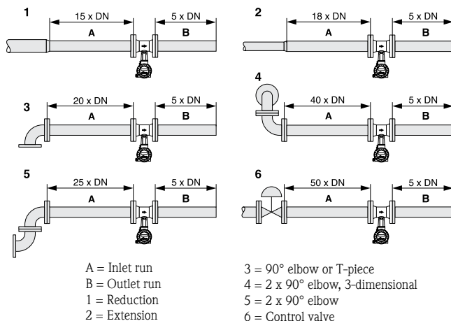
Figure 2: Inlet and outlet runs
