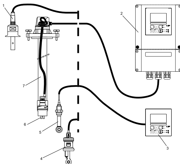
Figure 3: Example of a complete measuring system
