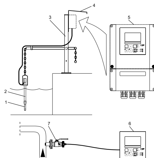
Figure 1: Examples of complete measuring systems
